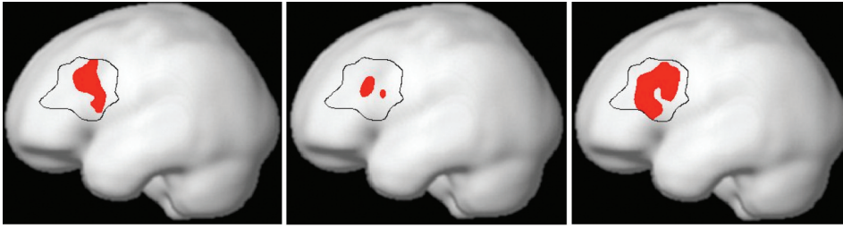
Brain activations of the left frontal language area (shown in red) varies considerably between three subjects.
