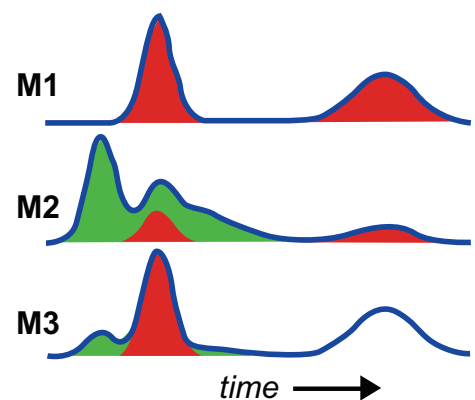
Graphic illustrating how two modules (shown in green and red) can control complex patterns of activity in three muscles (M1, M2, and M3).
